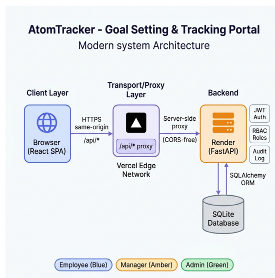
Figure 1 — Browser -> Vercel Proxy -> FastAPI (Render) -> SQLite Component Breakdown
