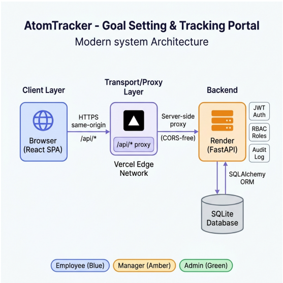
Figure 1 — Browser -> Vercel Proxy -> FastAPI (Render) -> SQLite
