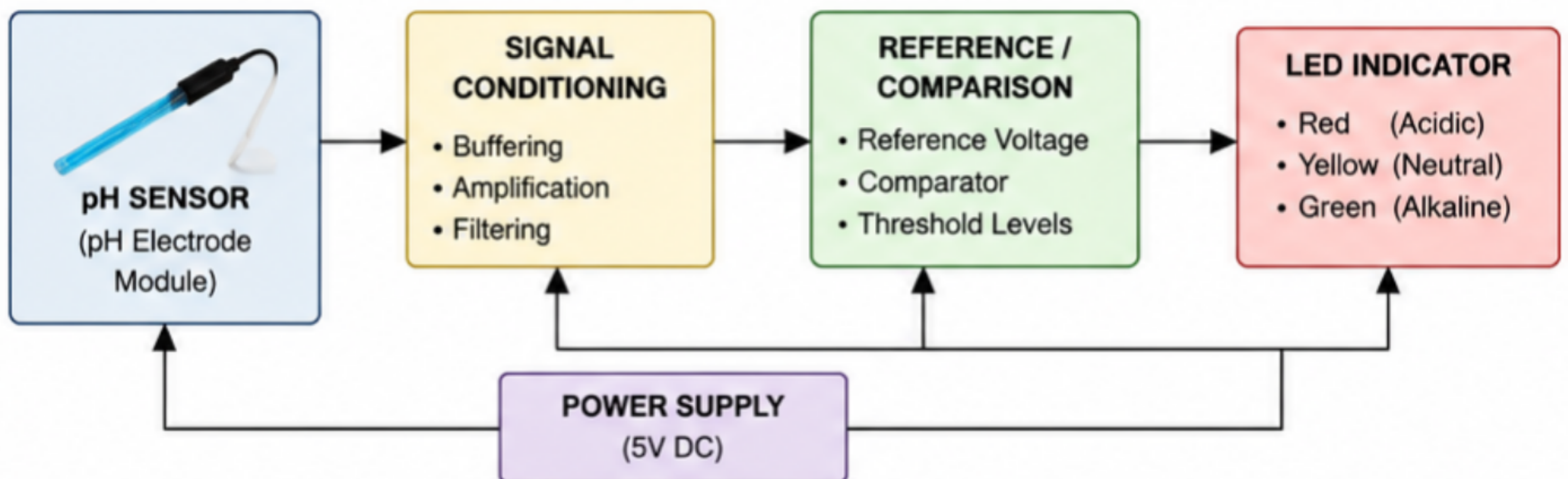
Proposed System Block Diagram
