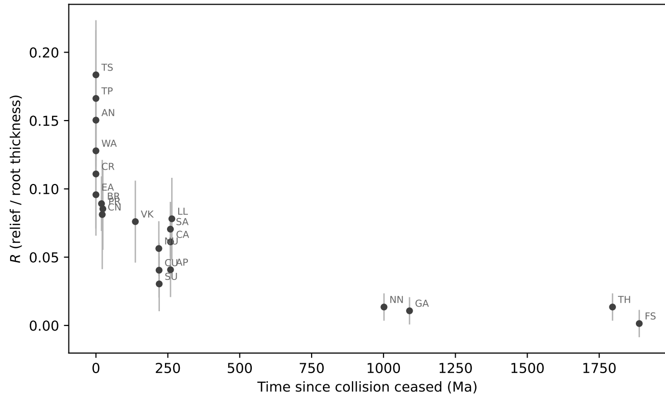
Root buoyancy ratio vs. orogen age (digitized from Fischer et al.)
