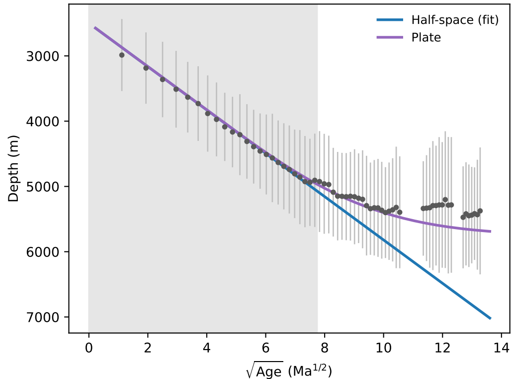
Linearized: depth vs. \sqrt{\text{age}}
