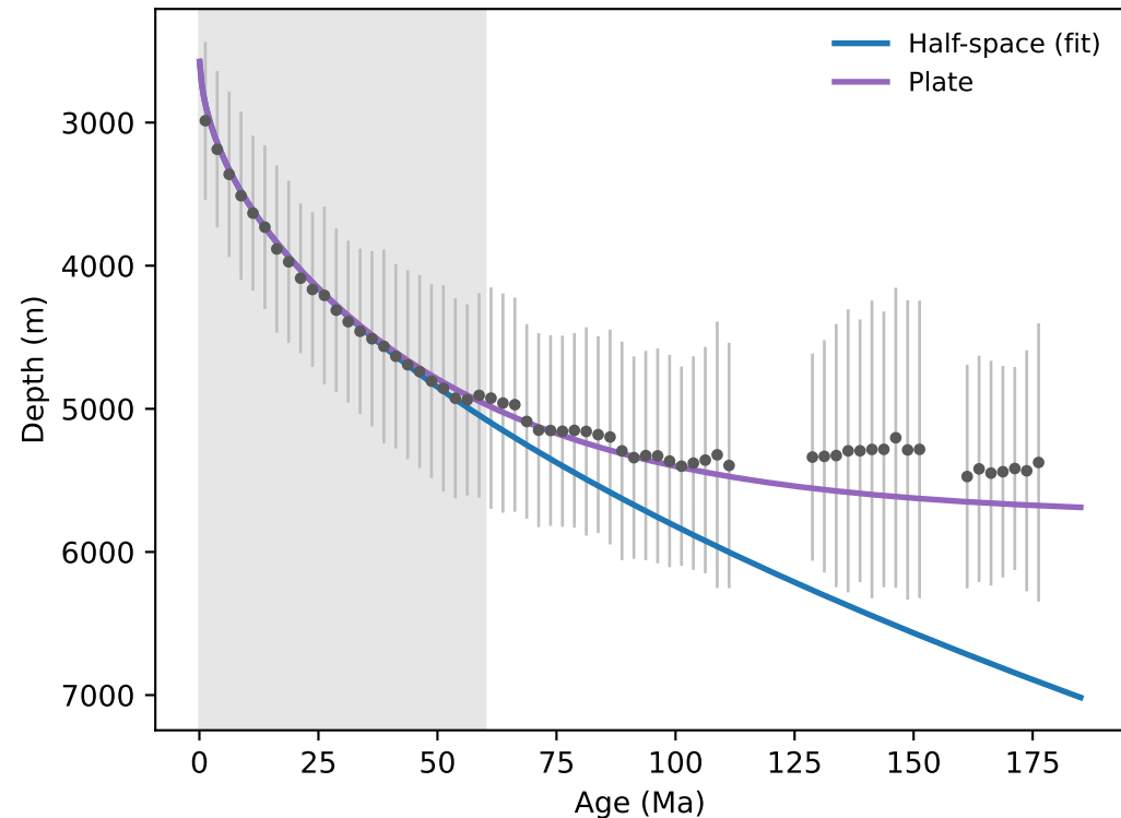
Bathymetry vs. age
