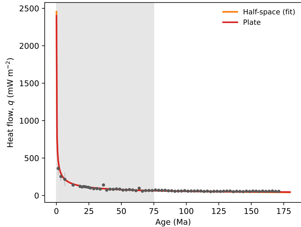
Heat flow vs. age
