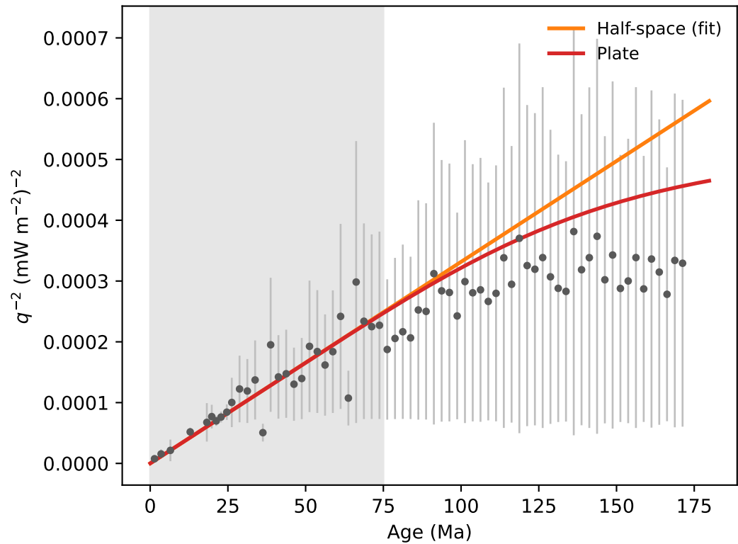
Linearized: q^{-2} vs. age
