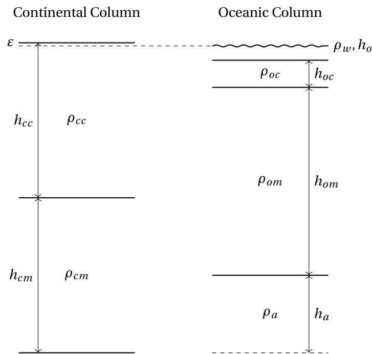
Figure 8: Comparison of isostatic columns for the continental and oceanic crust for Part B.
