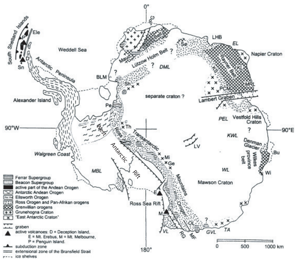
Figure 11: Tectonic map of Antarctica from Talarico and Kleinschmidt ( Antarctic Climate Evolution , 2008).
