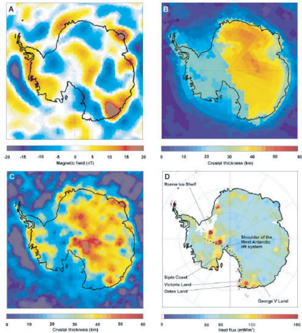
Figure 10: Estimating the Curie depth from vertical magnetic data. (a) Vertical magnetic field. (b) Crustal thickness model of Antarctica. (c) Estimate to base of magnetized layer. (d) Estimated heat flow. Figure from Maule et al. ( Science , 2005).
