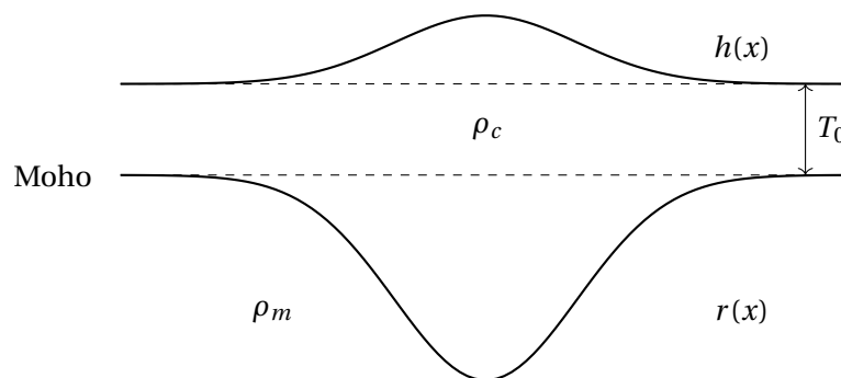
Figure 9: A mountain with a topographic expression h(x) and compensating root r(x) .
