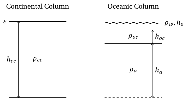
Figure 7: Comparison of isostatic columns for the continental and oceanic crust for Part A.
