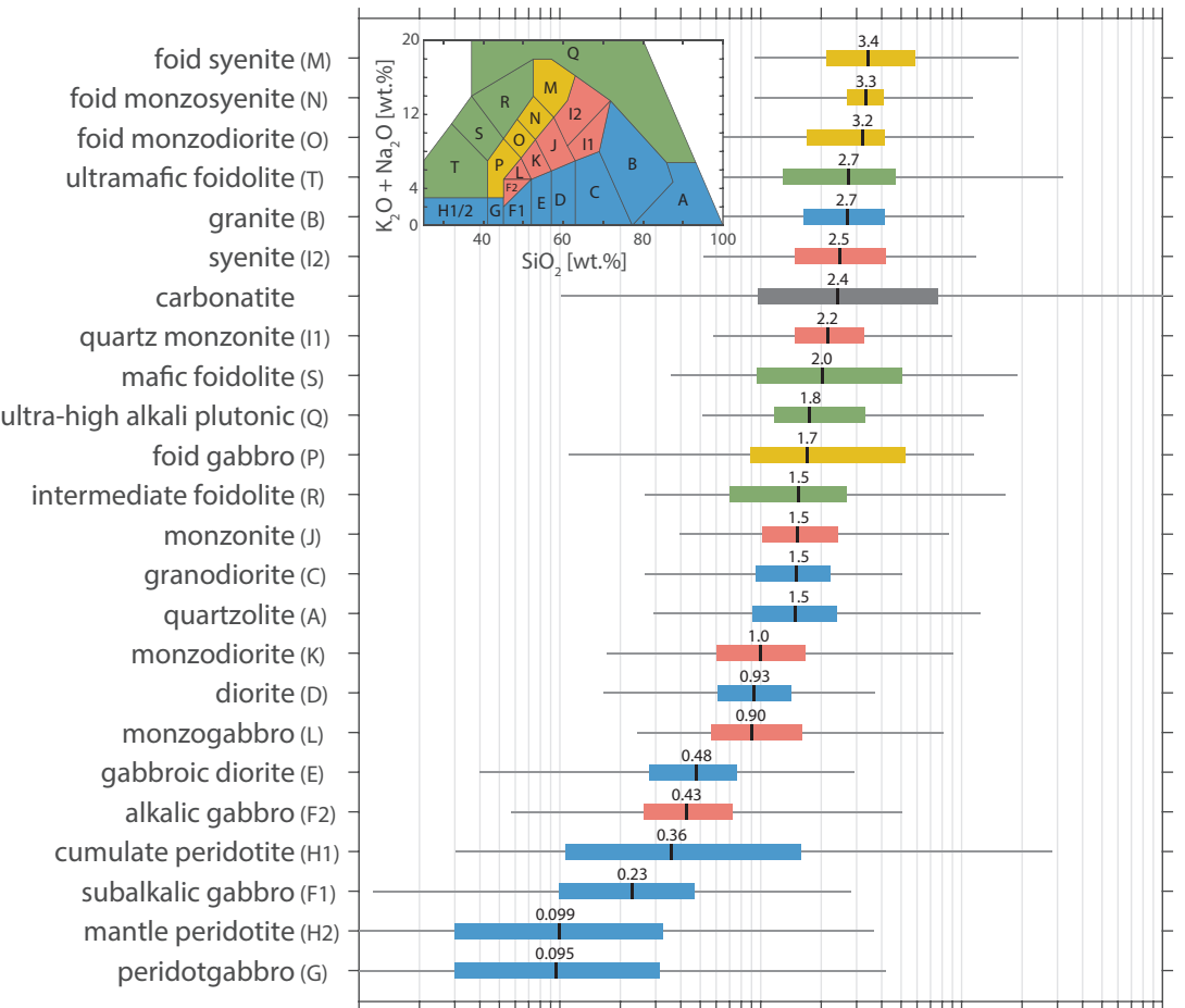
(a) Igneous Plutonic
