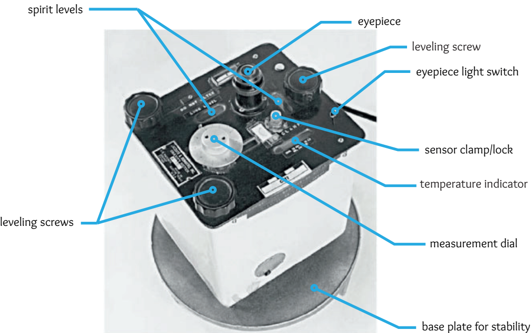
Anatomy of a Gravimeter
