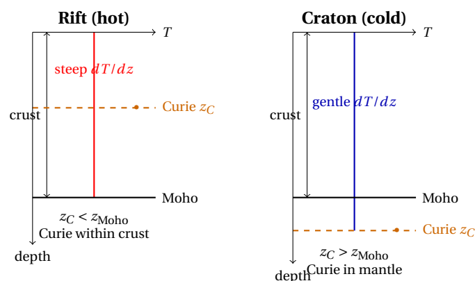
Figure 5: In a rift (hot, steep geotherm) the Curie isotherm lies within the crust. In a craton (cold, gentle geotherm) it may lie below the Moho. Seismic and magnetic crustal thickness therefore differ systematically between tectonic settings.
