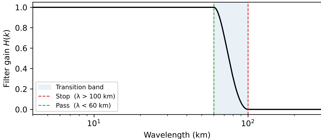
Raised-cosine high-pass filter response
