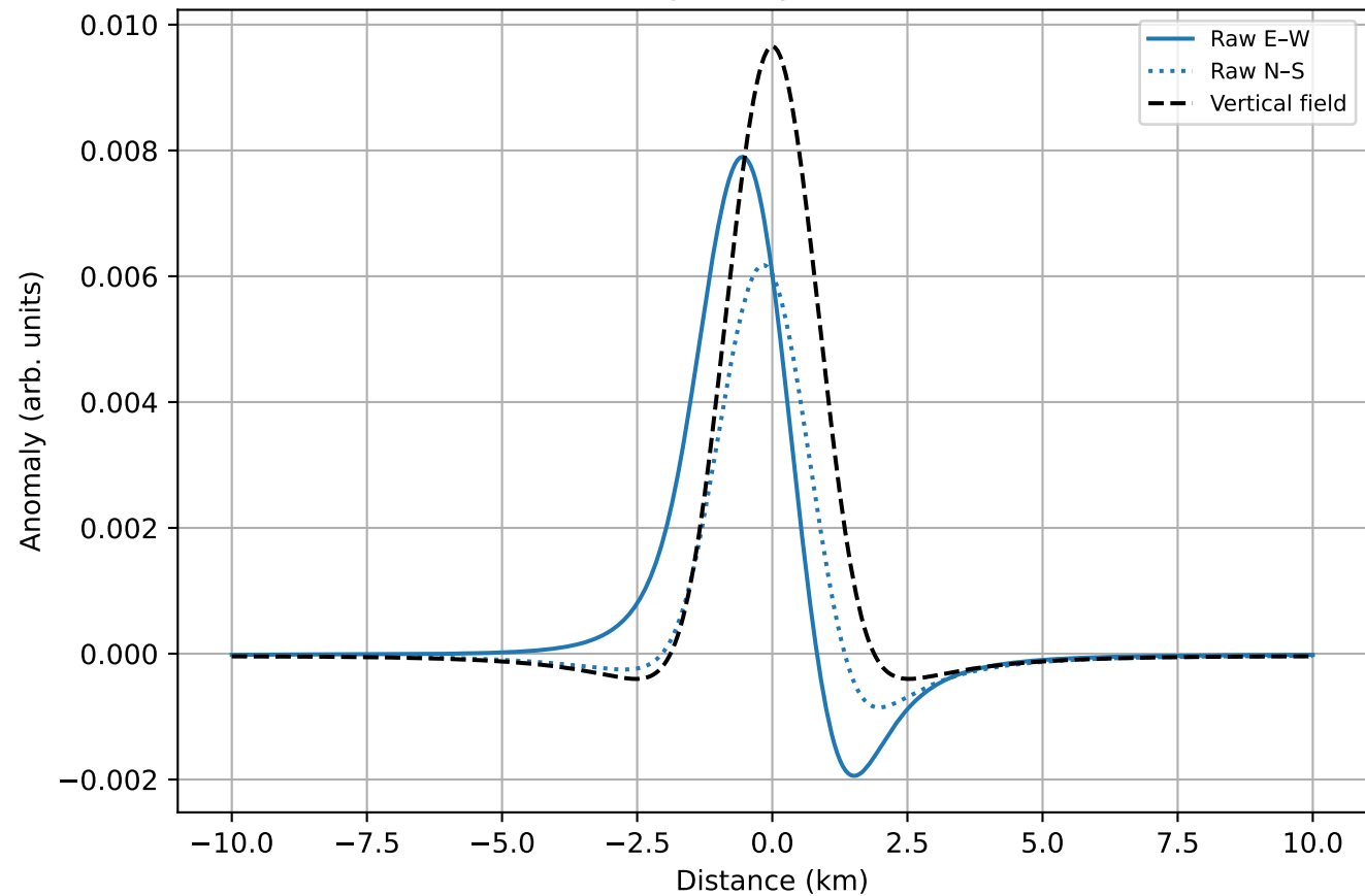
Cross-sections through body centre — I=60^\circ , D=15^\circ
