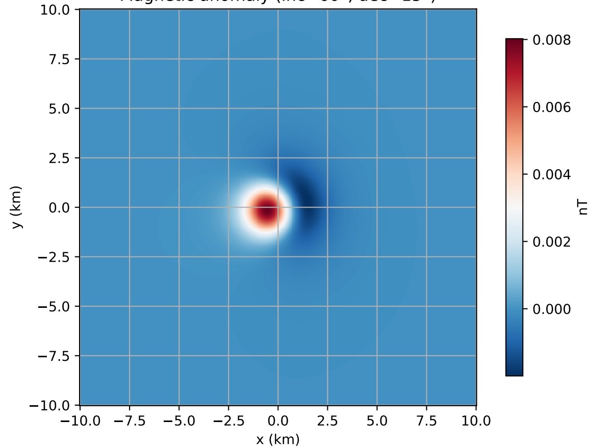
Magnetic anomaly (inc=60°, dec=15°)
