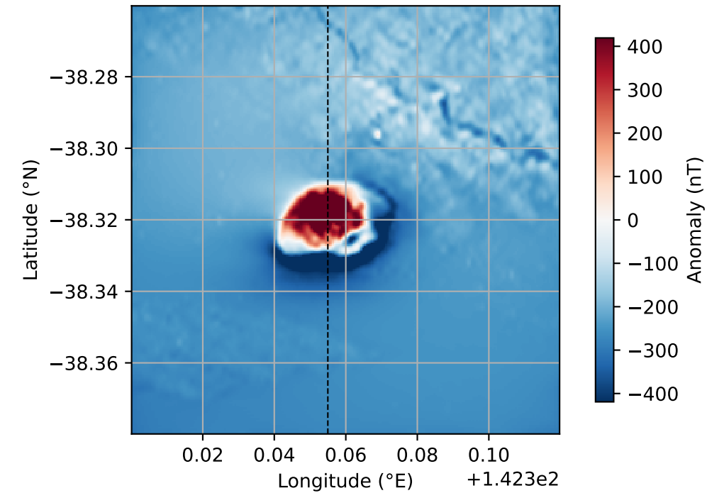
Tower Hill — RTP (Inc=-70°, Dec=10.5°)
