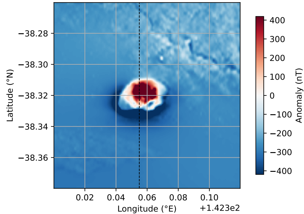
Tower Hill — Magnetic anomaly (IGRF removed)
