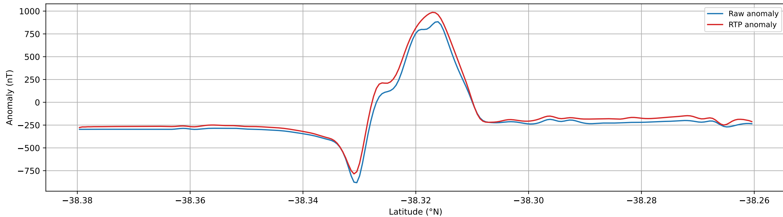
N-S cross-section at Lon \approx 142.3550^\circ\text{E}
