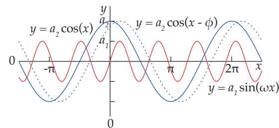
Sine and Cosine
