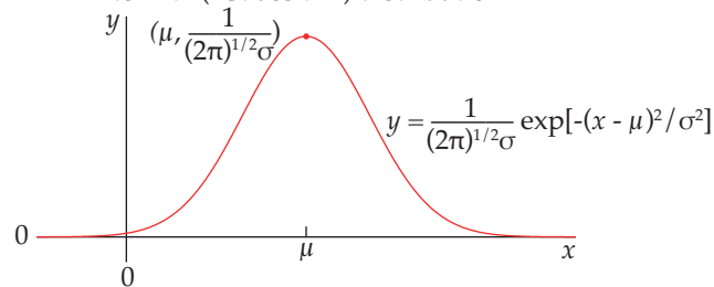
Normal ("Gaussian") distribution
