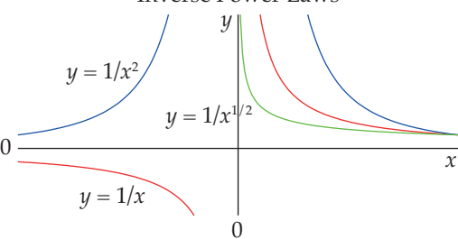
Inverse Power Laws
