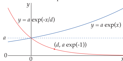
Exponential
