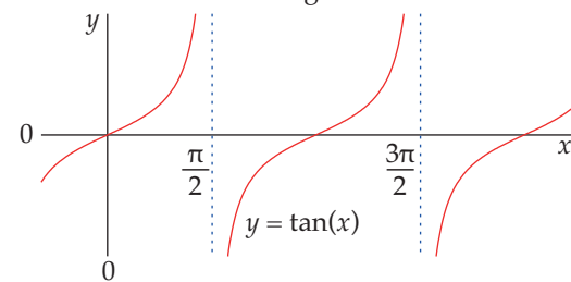
Tangent
