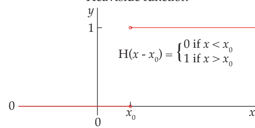
Heaviside function
