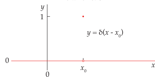
Delta function
