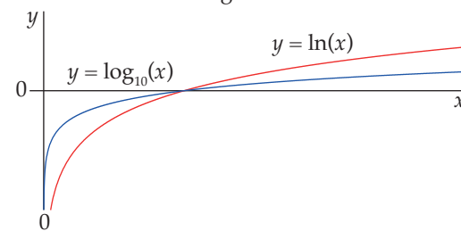
Logarithm
