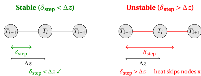
Figure 4: Stability requires that the thermal \delta_{\text{step}} = \sqrt{2\kappa\Delta t} does not exceed the node spacing \Delta z . When it does, heat is asked to propagate past neighboring nodes in one step, which is physically impossible and causes numerical blow-up.
