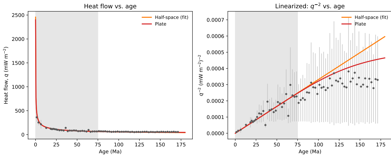
Figure 2: Sediment-corrected global heat flow vs. seafloor age (binned, error bars show one standard deviation). The half-space curve here is fit by least squares to every point in the shaded region ( t < 75 Ma), giving c_q \approx 549 \text{ mW m}^{-2} \text{ Ma}^{1/2} .
