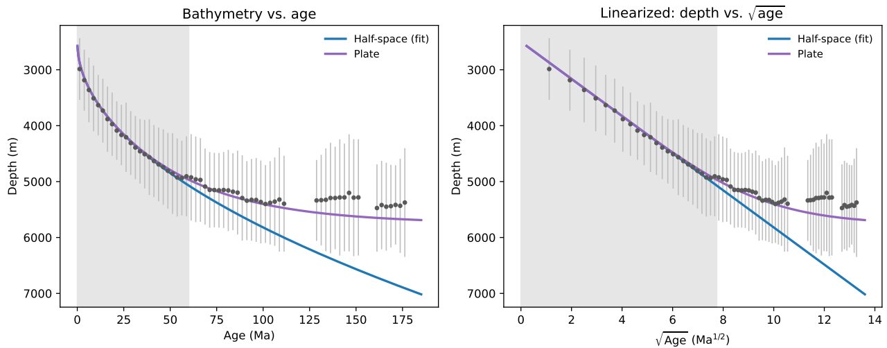
Figure 3: Global bathymetry vs. seafloor age (binned, error bars show one standard deviation). The half-space curve is fit to every point in the shaded region ( t < 60 Ma), giving c_s \approx 332 \text{ m Ma}^{-1/2} .
