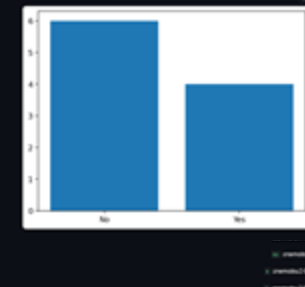
Churn Distribution
