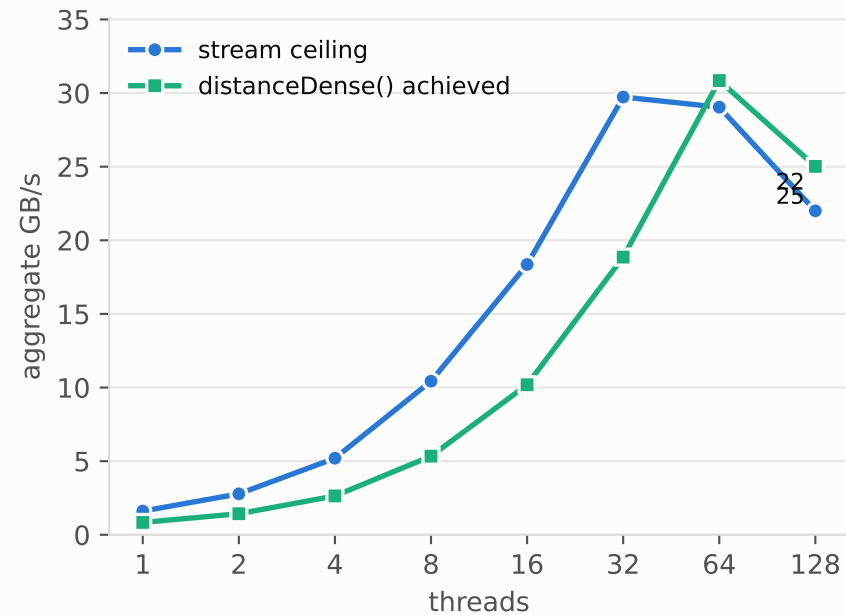
Achieved vs Achievable Bandwidth
