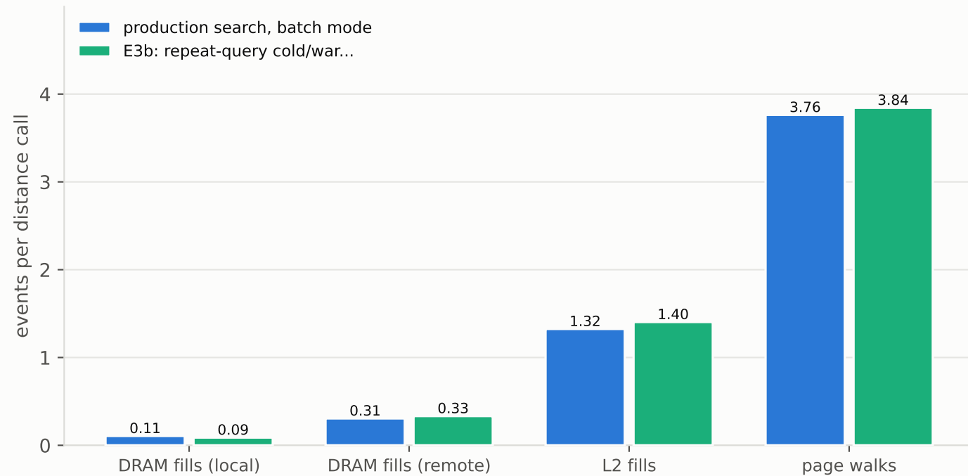
Memory events per distance call
