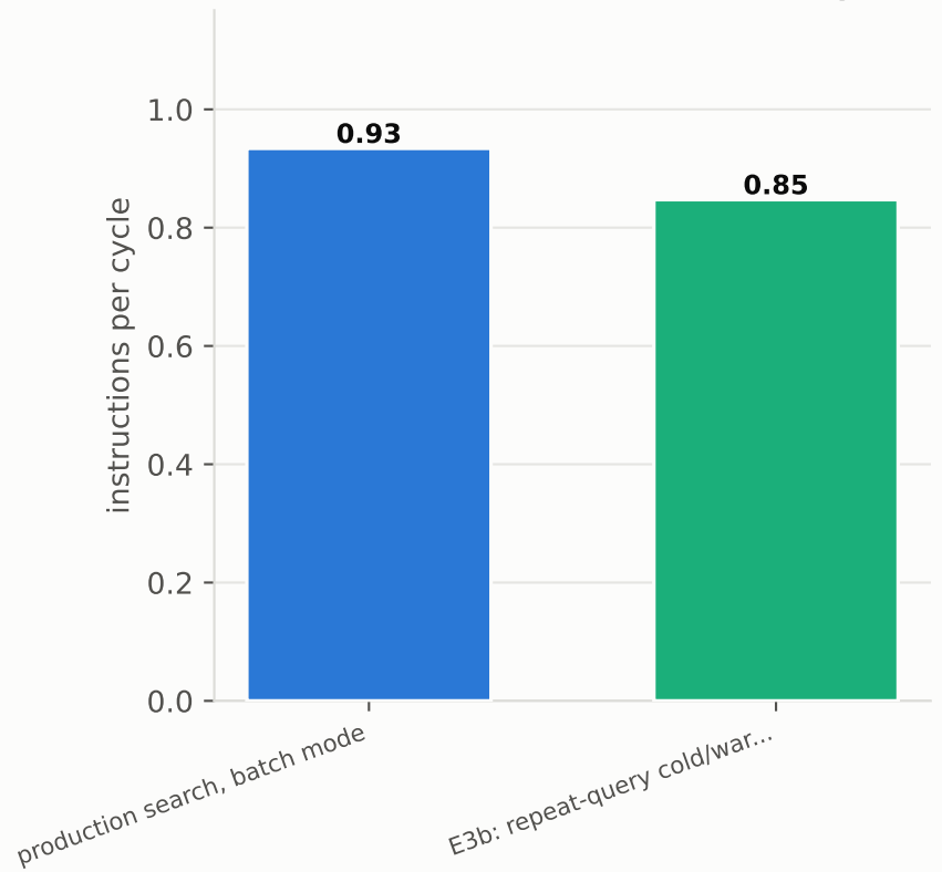
IPC (low = stalled on memory)
