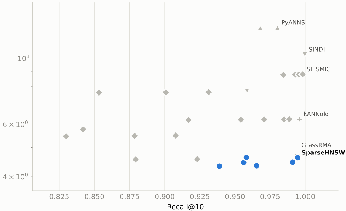
Memory Cost vs Recall
