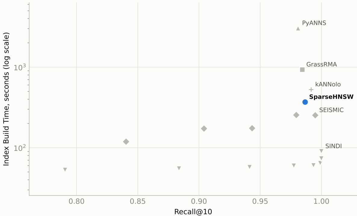
Index Build Cost vs Recall
