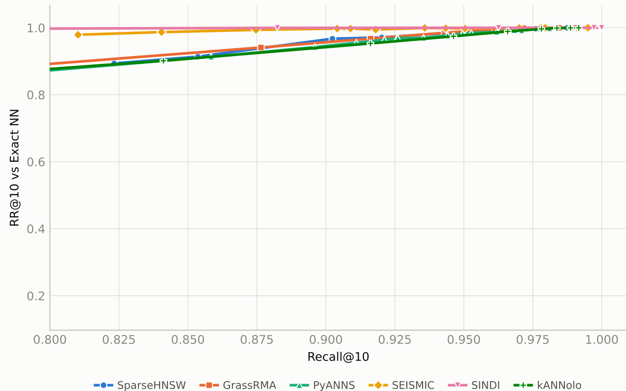
Ranking Quality vs Recall
