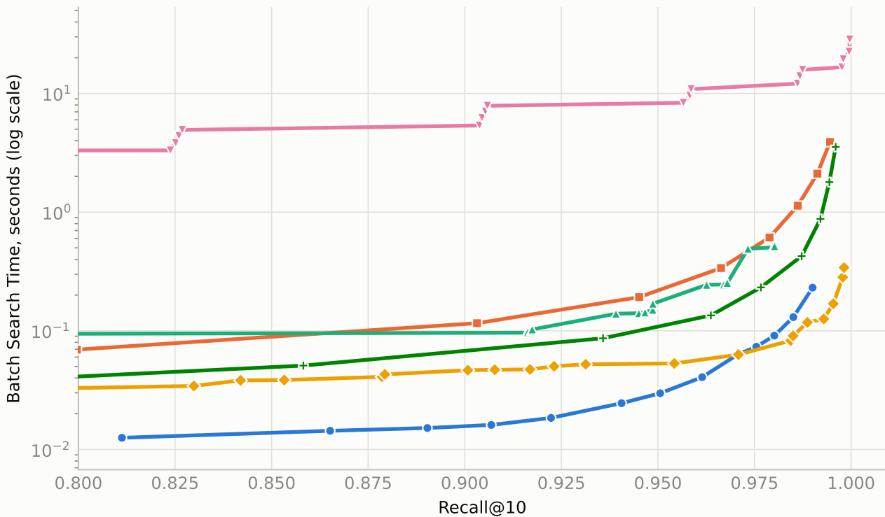
Search time vs Recall
