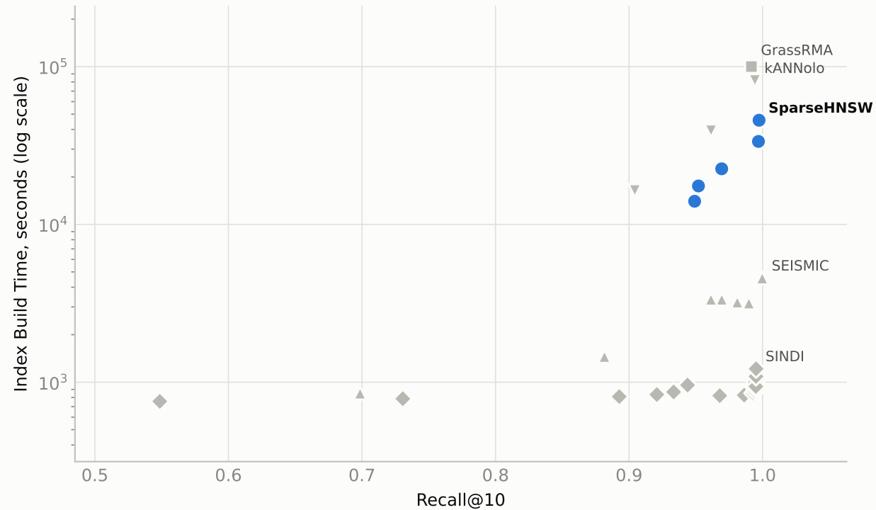
Index Build Cost vs Recall
