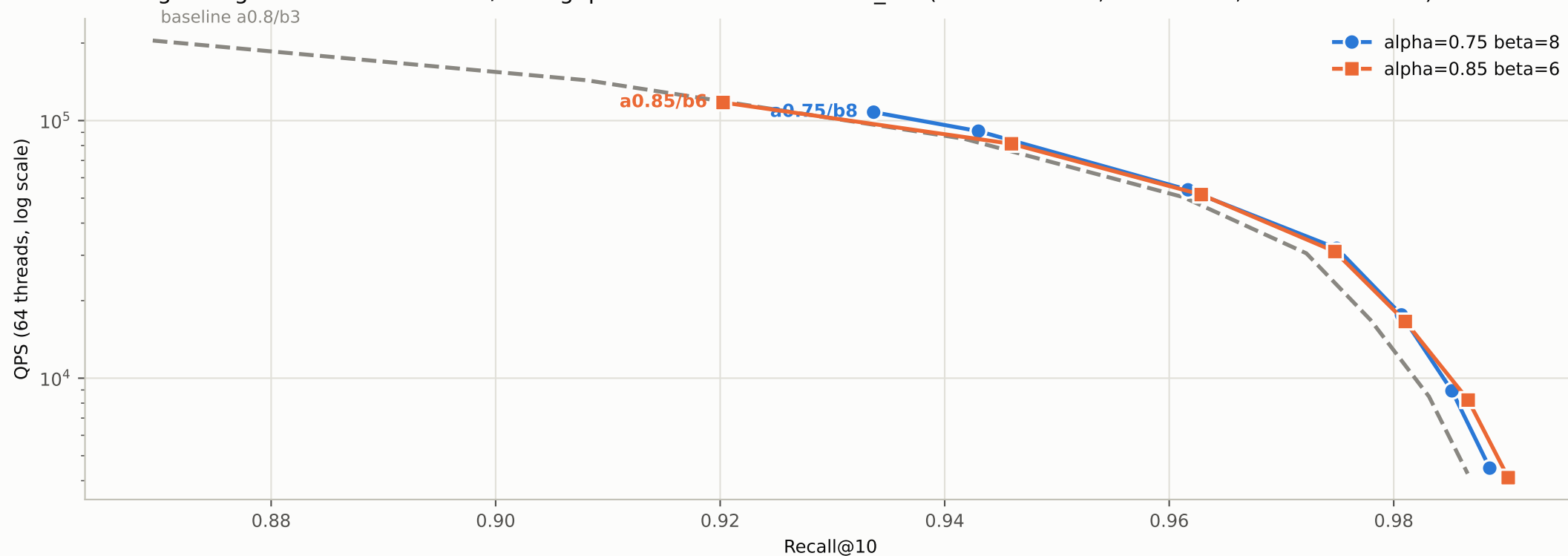
Pruning configurations on the recall/throughput frontier — msmarco_full (8841823 docs, 64 threads, M=32 efC=200)
