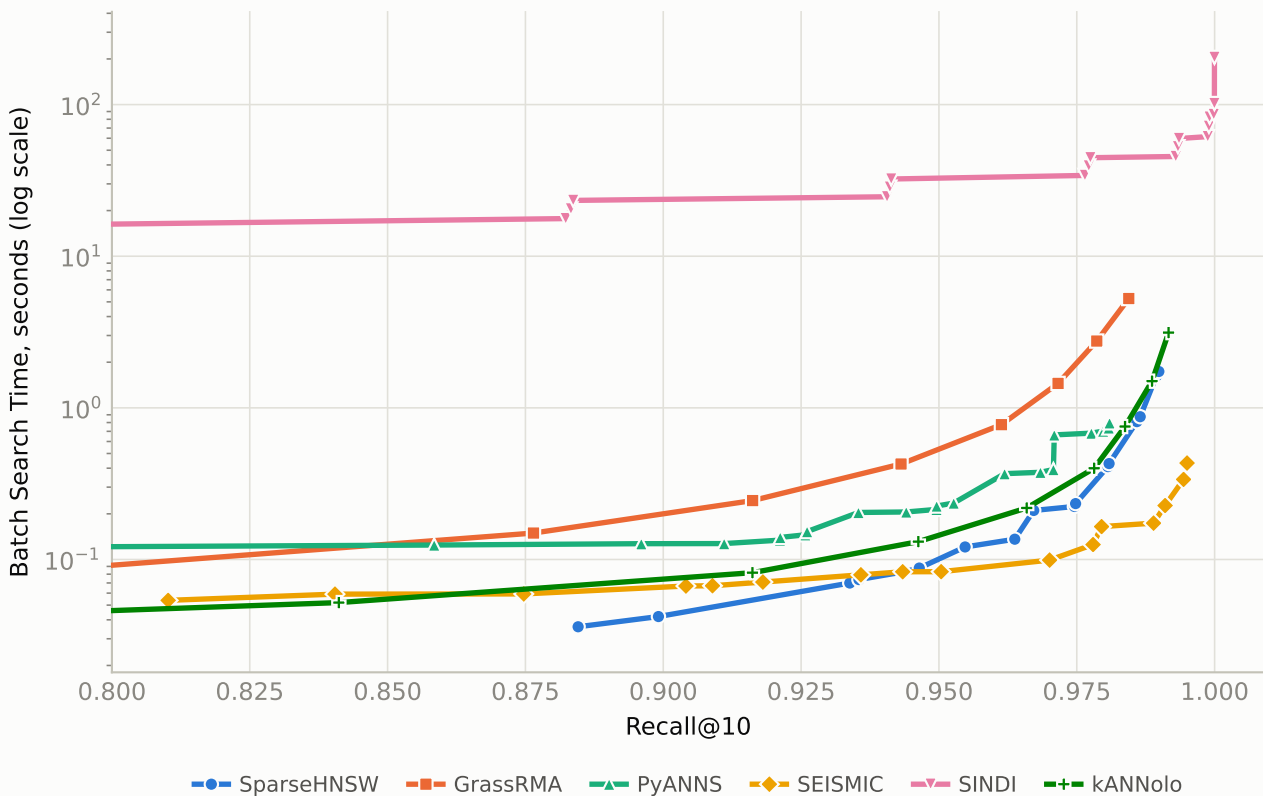
Search time vs Recall
