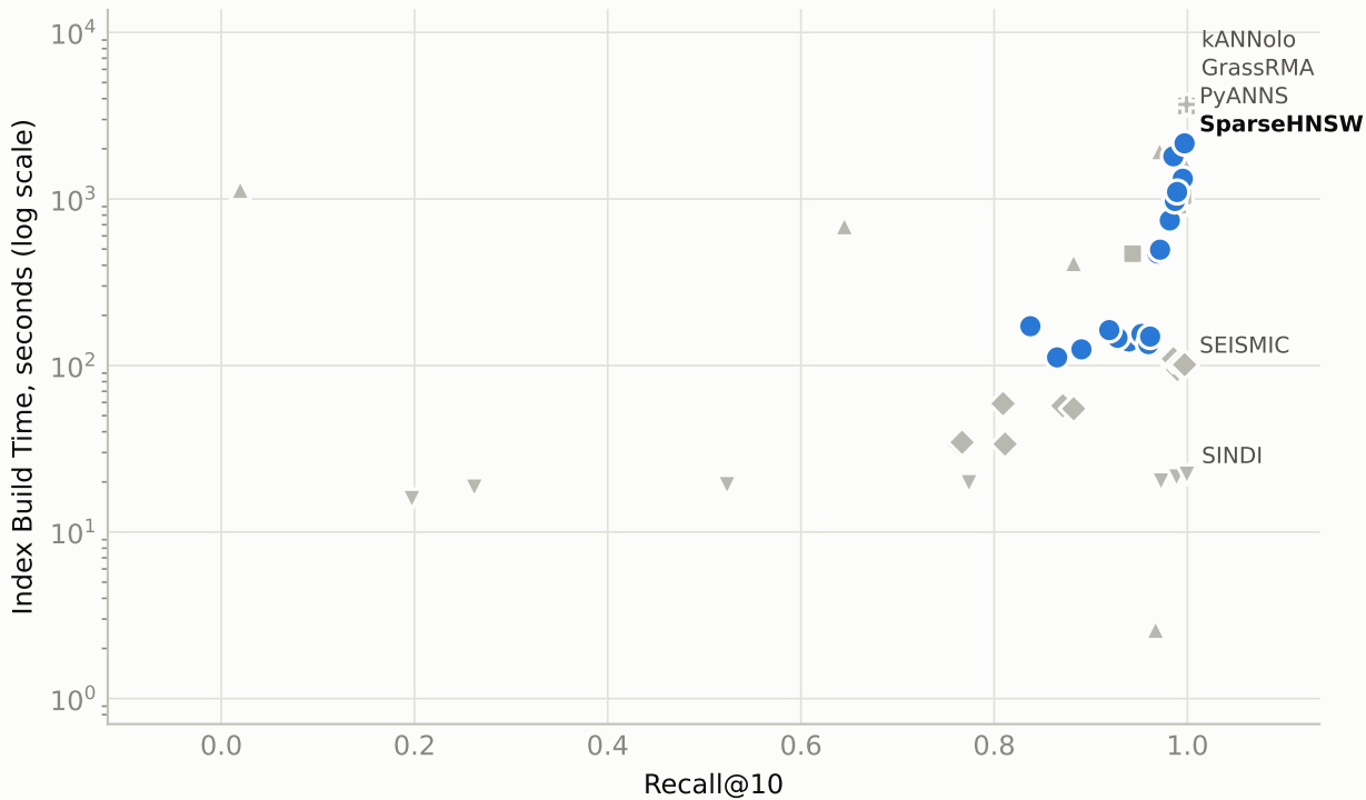
Index Build Cost vs Recall
