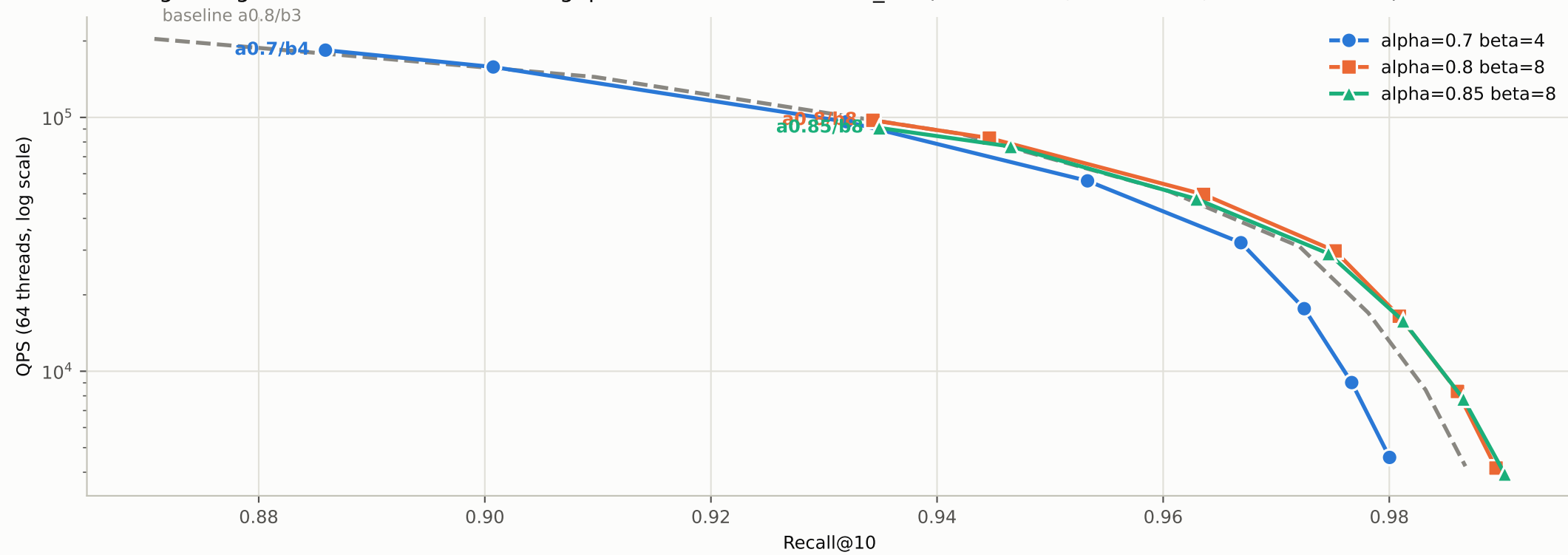
Pruning configurations on the recall/throughput frontier — msmarco_full (8.84M docs, 64 threads, M=32 efC=200)
