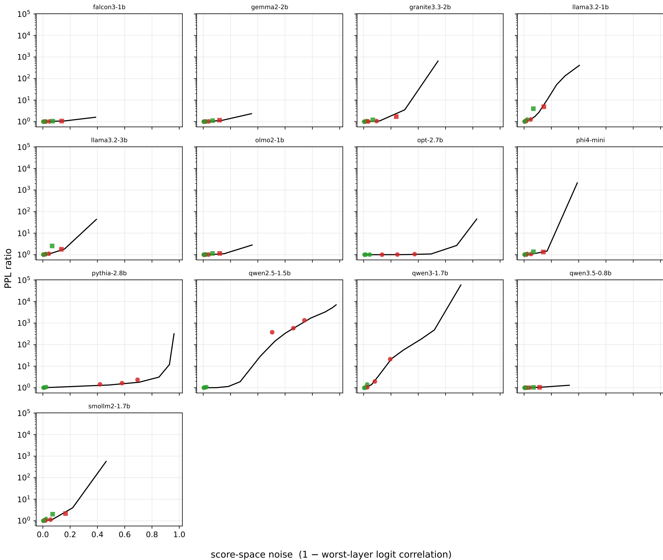
Damage is a model-specific function of one scalar: each model's noise curve (line, measured with Gaussian noise and no quantizer) vs its quantizer cells (red=uncentered, green=centered, square=1-bit)
