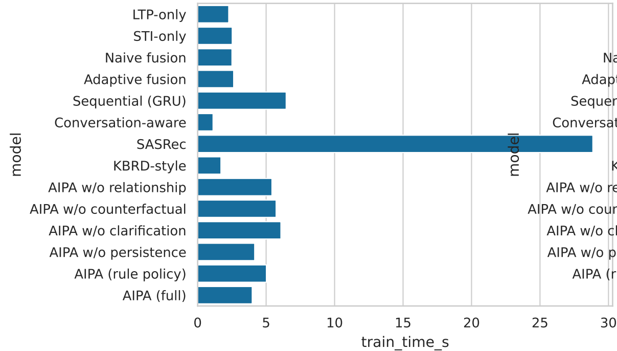
Training time (s, mean over seeds)
