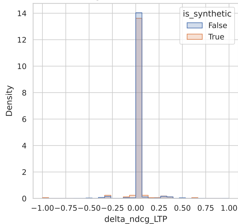
\Delta NDCG@10 when LTP is neutralised
