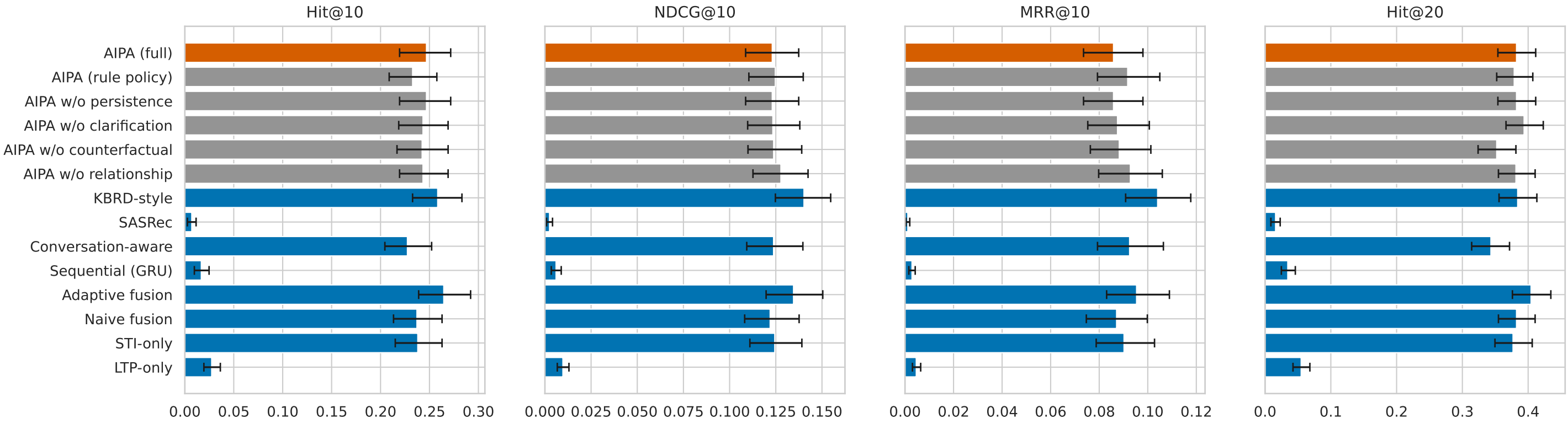
Synthetic Conflict/Override subset (n=226; bars = mean over seeds, whiskers = 95% bootstrap CI)
