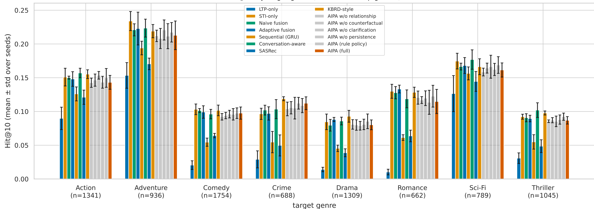
Hit@10 by target genre (natural test, top genres)
