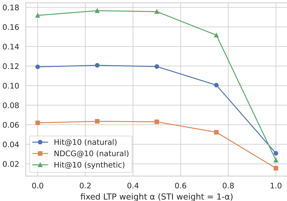
Fixed fusion weight sweep (Naive-fusion encoders)
