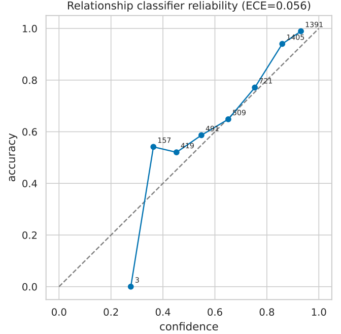
Fig. 8. Reliability diagram of the relationship head.
