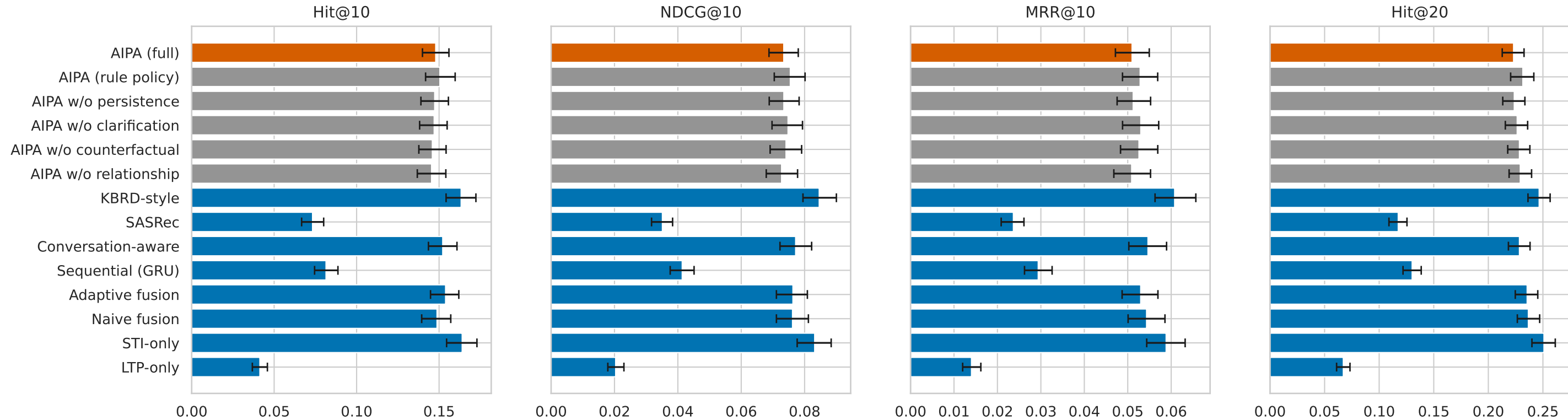
Natural conflict subset (broad) (n=1272; bars = mean over seeds, whiskers = 95% bootstrap CI)
