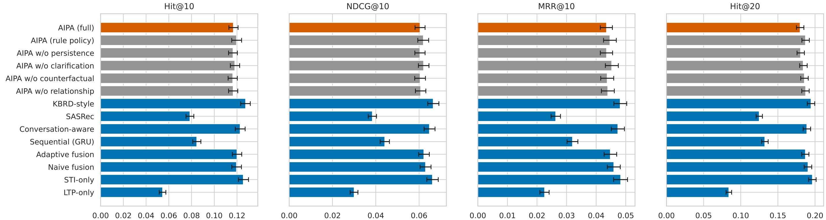
Natural test instances (n=4472; bars = mean over seeds, whiskers = 95% bootstrap CI)
