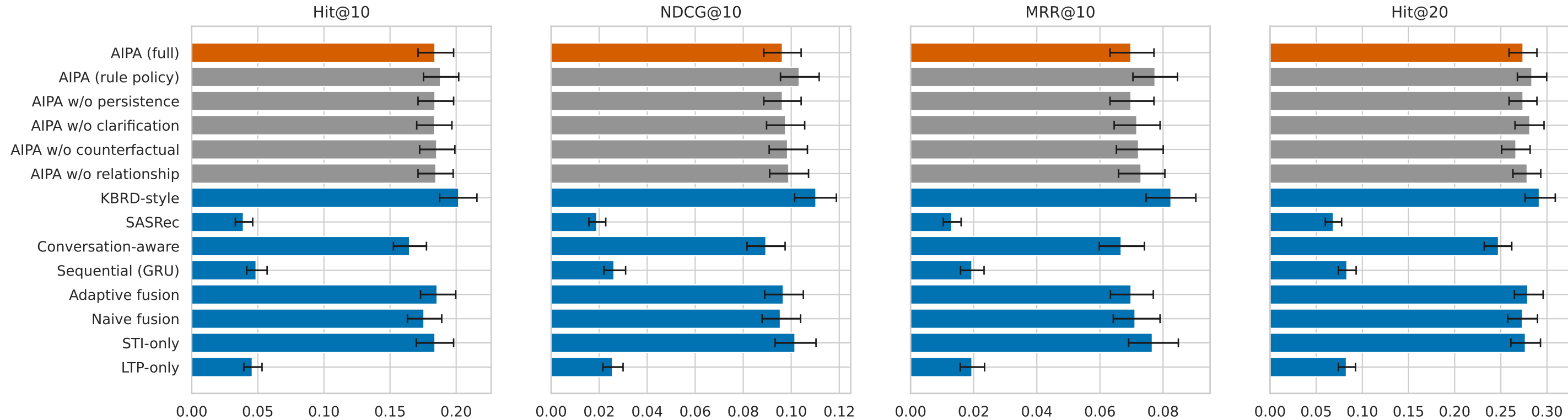
Controlled synthetic test instances (n=624; bars = mean over seeds, whiskers = 95% bootstrap CI)
