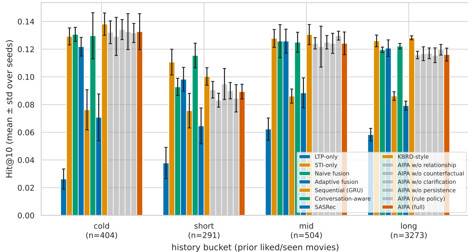
Hit@10 by LTP history length (natural test)
