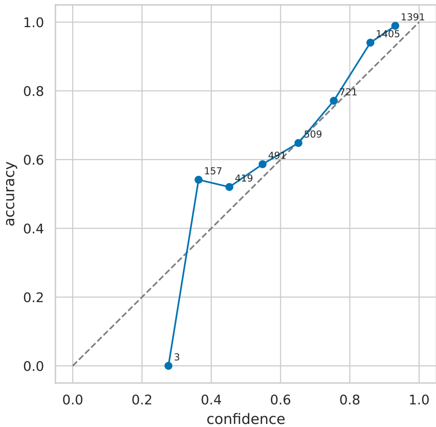
Relationship classifier reliability (ECE=0.056)
