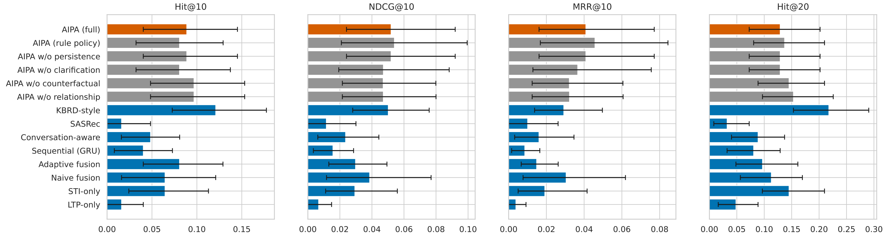
Natural conflict subset (strict) (n=62; bars = mean over seeds, whiskers = 95% bootstrap CI)
