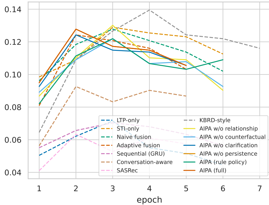
Validation Hit@10
