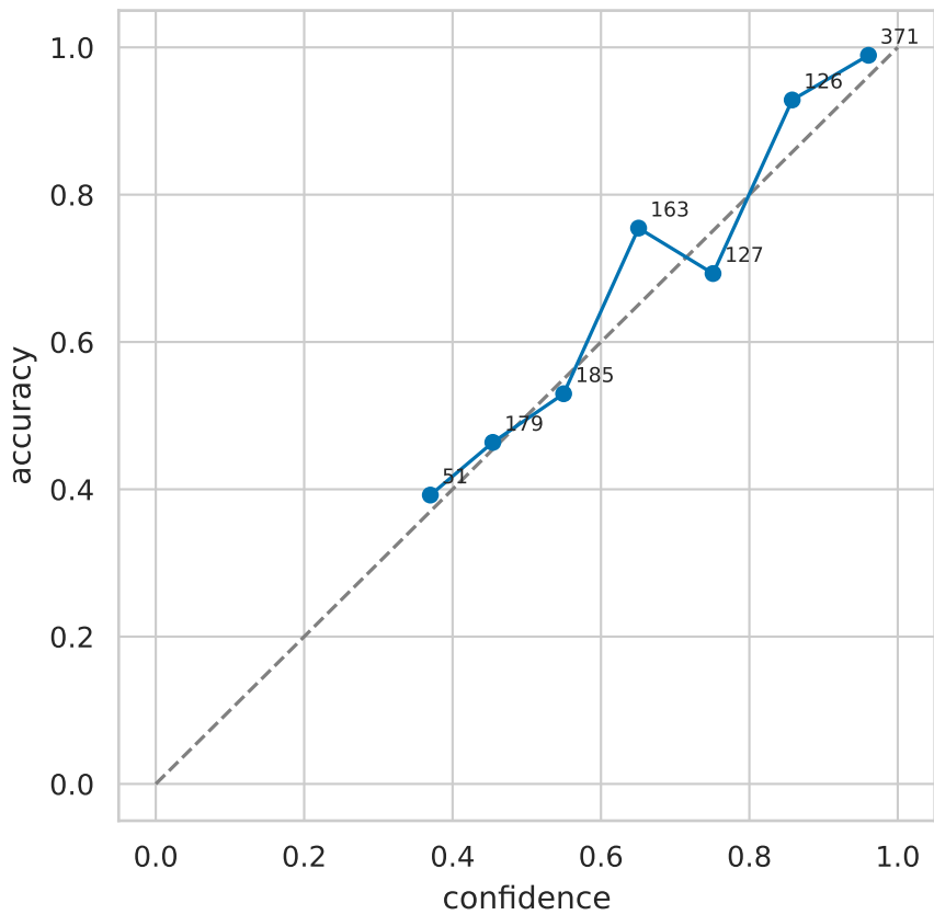
Relationship classifier reliability (ECE=0.042)
