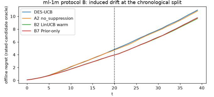
Fig. 9. Cumulative offline regret under protocol B on MovieLens-1M. The dotted line is the induced switch round at T/2 .
