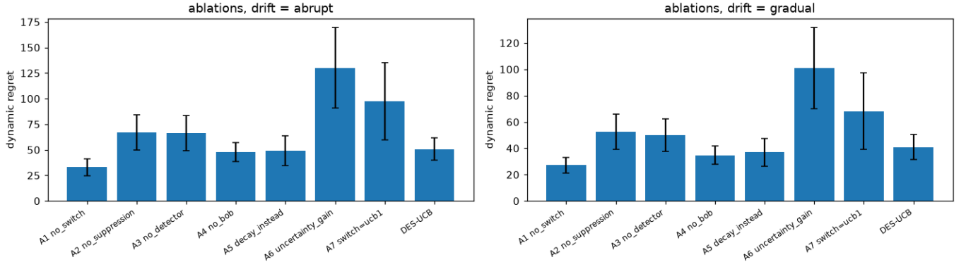
Fig. 6. Ablation dynamic regret on abrupt and gradual drift. Bars are means over units and whiskers are one standard deviation.
