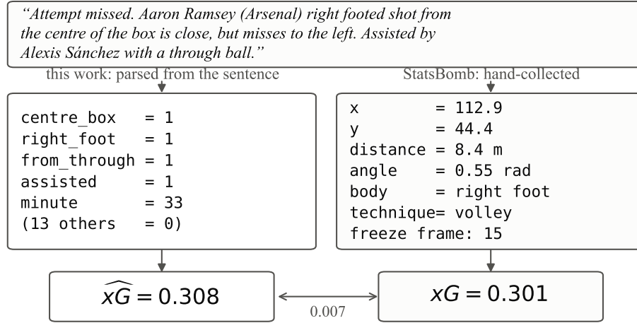
Fig. 1. The same shot as each side of the comparison receives it. The commentary sentence yields eighteen parsed indicators and no geometry; the StatsBomb release yields a location, a derived distance and angle, and the positions of the players in view. Neither side sees the other’s representation, and both are scored against the same outcome.
