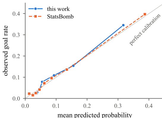
Fig. 2. Reliability of both models on the 8,825 joined shots, in octiles of predicted probability. The two curves lie almost on top of one another and both track the diagonal, so the gap in Table 3 is a difference in ranking rather than in calibration. Identity is carried by the legend and the marker shapes, since the curves coincide too closely to label in place.
