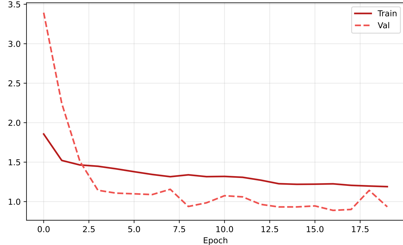
Loss
