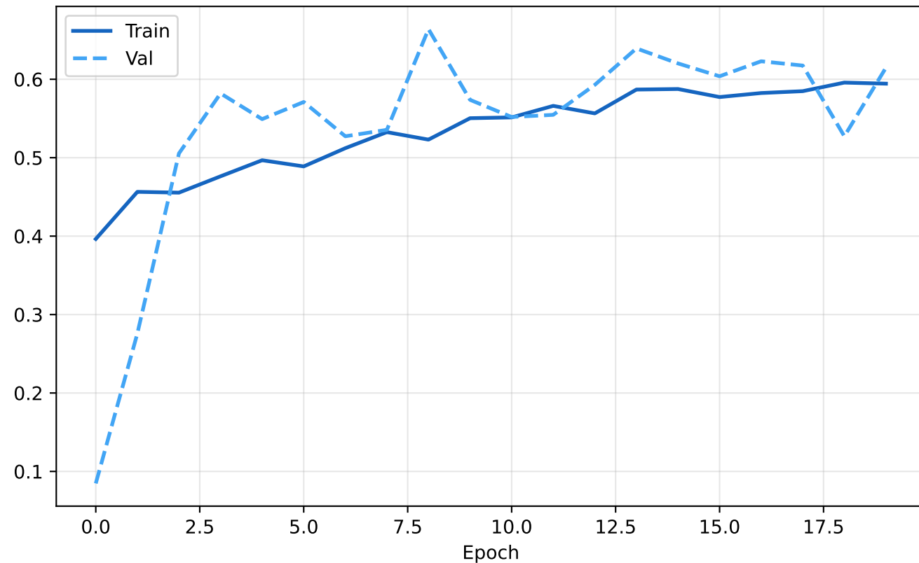
Accuracy
