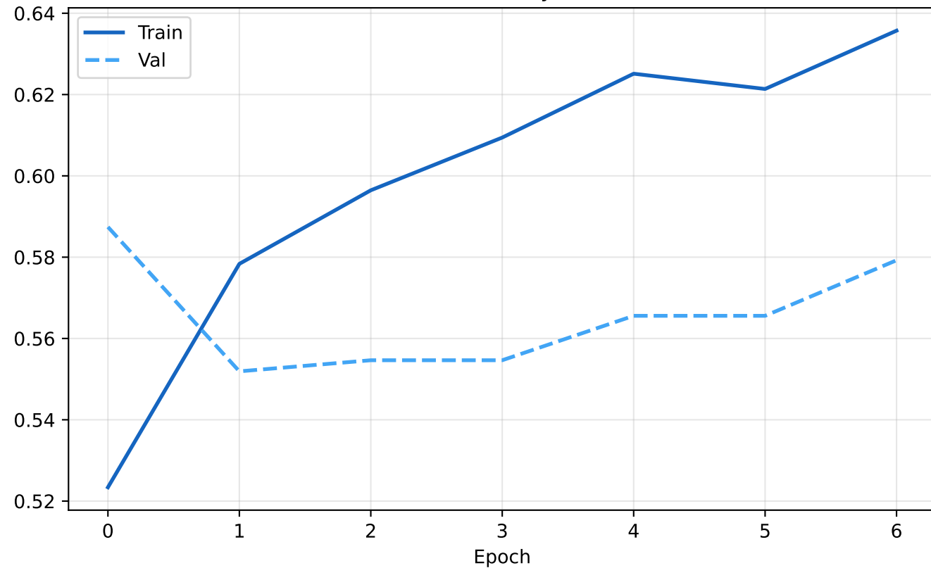
Accuracy
