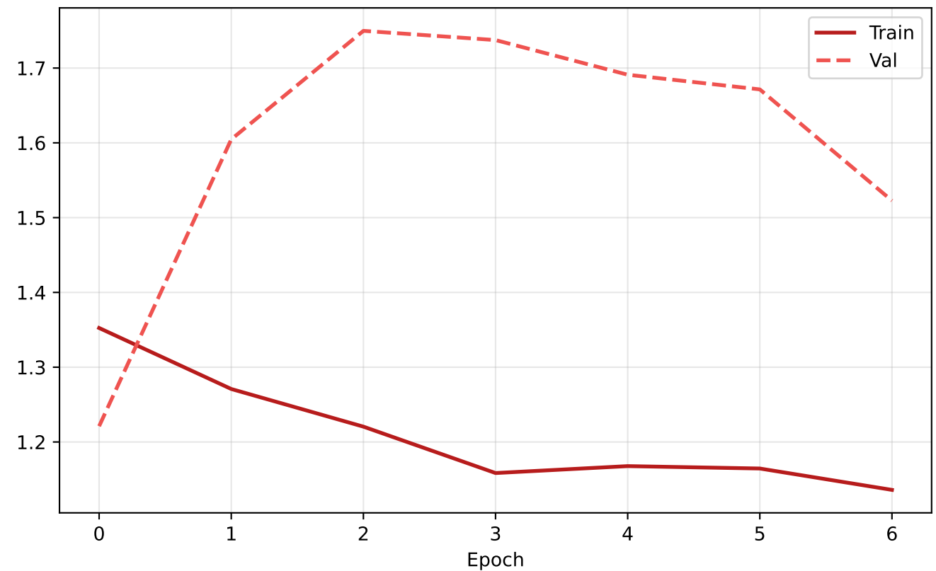
Loss
