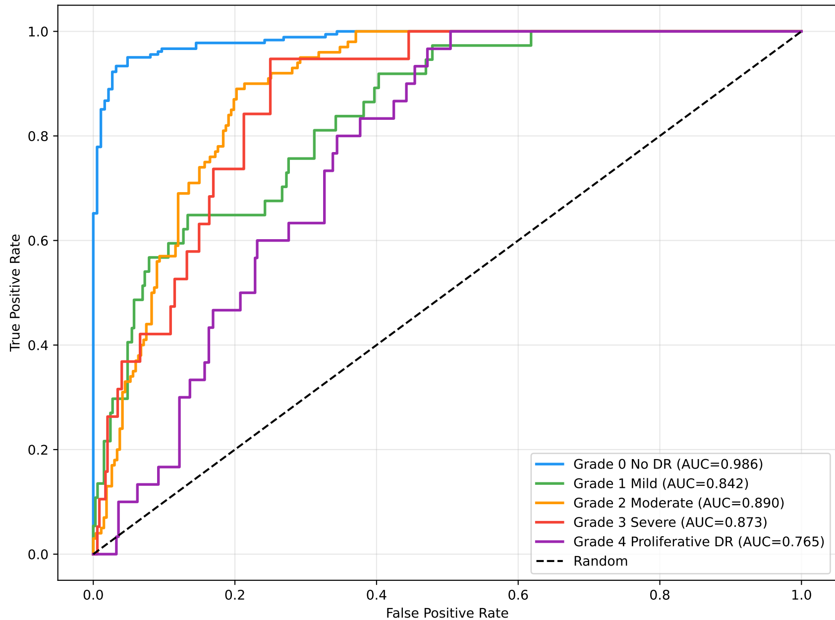
ROC Curves - ResNet50
