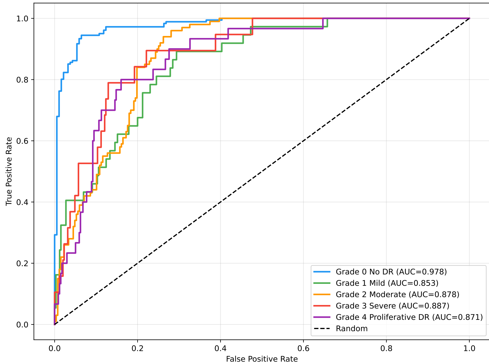
ROC Curves - MobileNetV2
