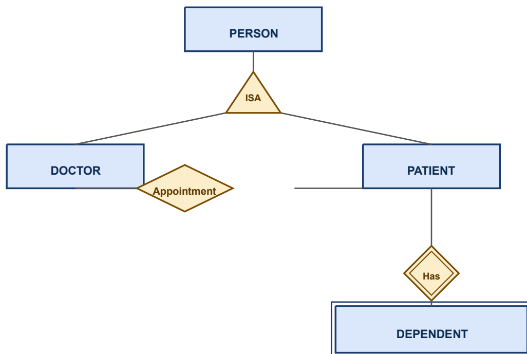
Fig. Q4 — EER Diagram of the Hospital Management System. PERSON generalizes DOCTOR and PATIENT (inheritance); DEPENDENT is a weak entity (double rectangle) linked to PATIENT via an identifying relationship (double diamond).
